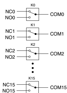
Figure 2. PXI-2566 Power-on State
