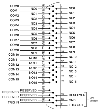
Figure 3. PXI-2566 Connector Pinout
